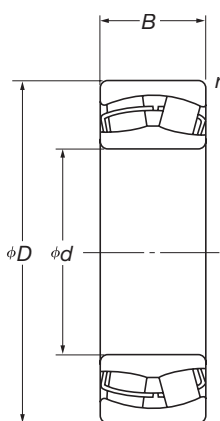
圆柱孔
